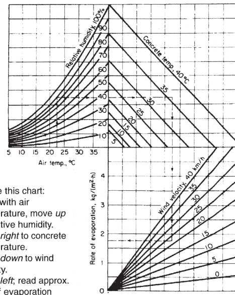
Fig. 12-9. Effect of concrete and air temperatures, relative humidity, and wind velocity on rate of evaporation of surface moisture from concrete. Reference 12-2.
